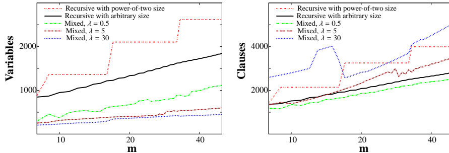
Fig. 4: Number of variables and clauses generated by Mixed and the Recursive Cardinality Networks approaches with input size 100 and different output sizes m .
