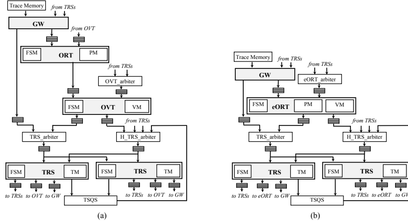
Figure 2: Task Superscalar hardware designs, a) base prototype, b) improved prototype
