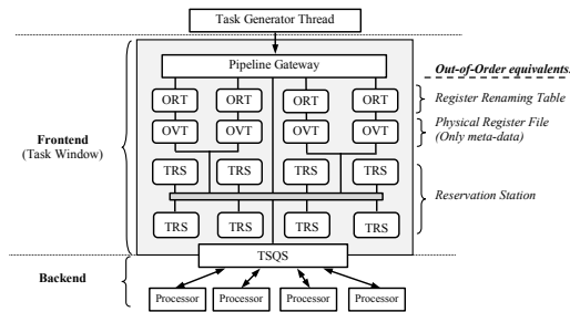
Figure 1: The Task Superscalar architecture
