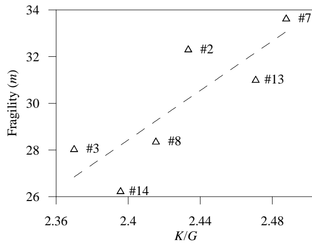
Fig. 3. Correlation between the fragility parameter m and the estimated ratio of the bulk to shear moduli K/G for the Ca-Mg-Cu glasses.
