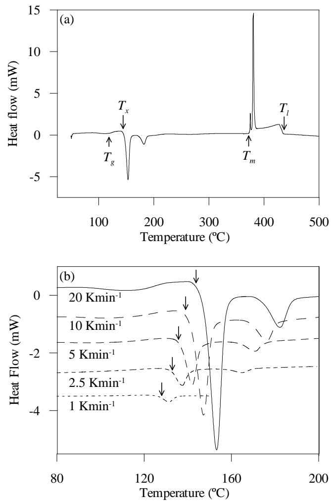
Fig. 1. (a) DSC curve for alloy 8 at Q = 20 \text{ K min}^{-1} . (b) DSC curves for alloy 8 at different heating rates.
