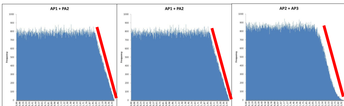
Fig. 2. Probability distributions for cases AP1 + AP2, AP1 + AP3 and AP2 + AP3, all with a denominator of 2.
