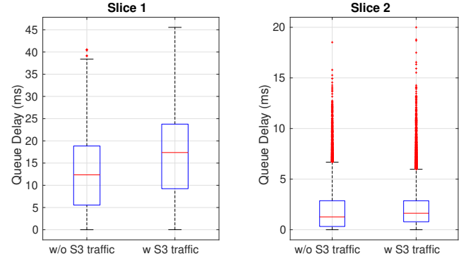
Fig. 3. Delay for Slices 1 and 2 with and without Traffic on Slice 3.
