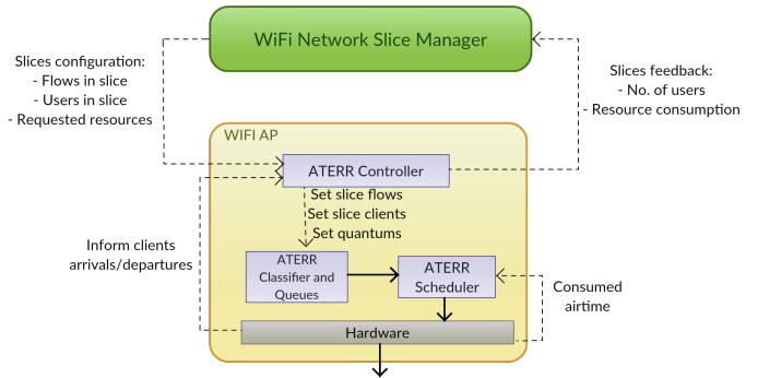
Fig. 1. ATERR Architecture.
