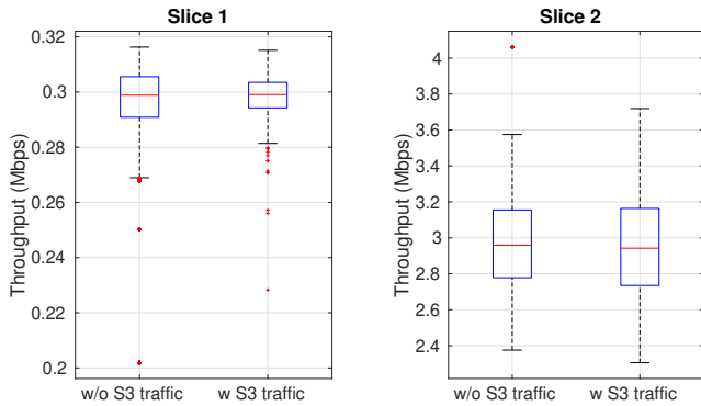
Fig. 4. Throughput for Slices 1 and 2 with and without Traffic on Slice 3.
