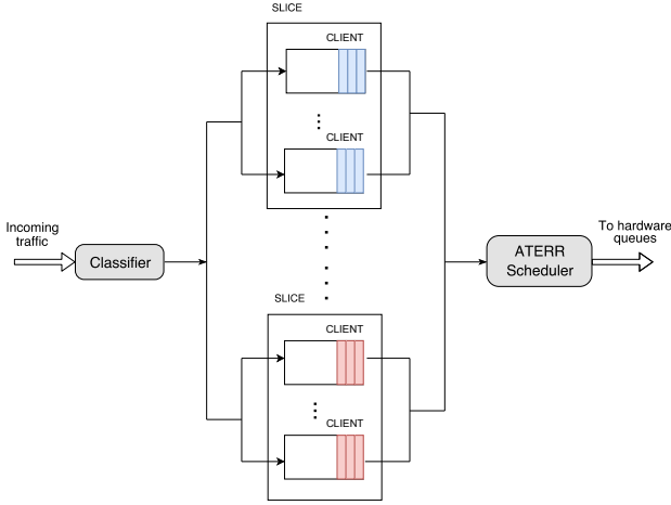
Fig. 2. ATERR Queuing Structure with the Classifier and the Scheduler.
