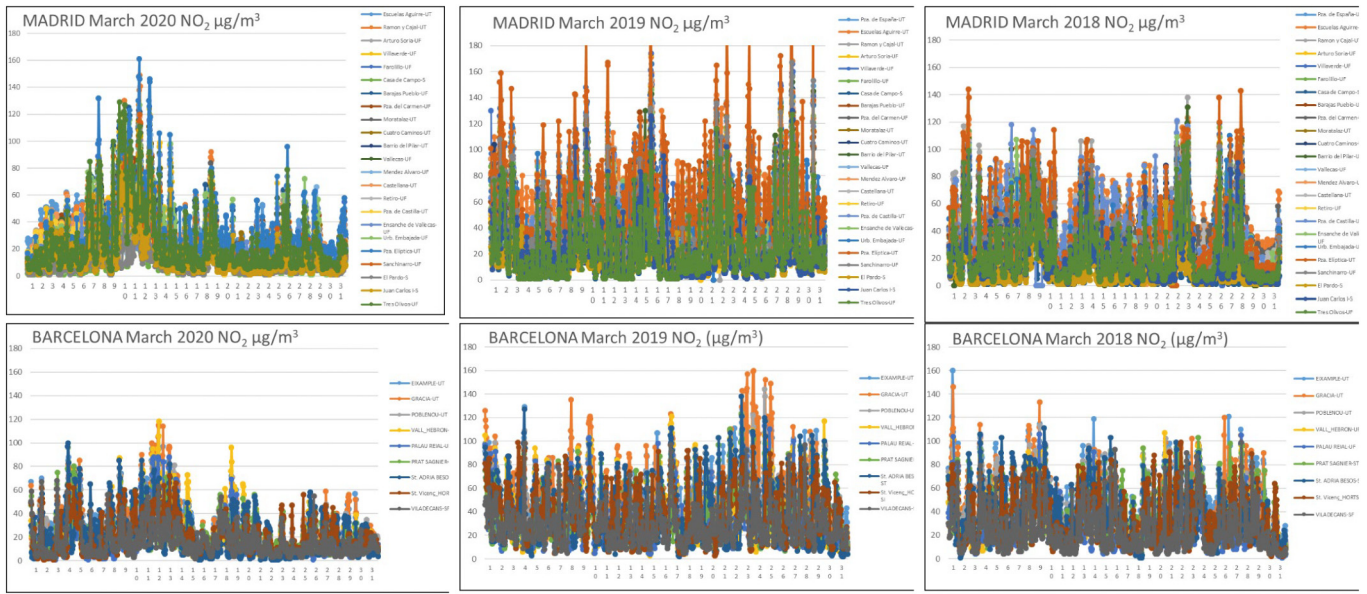
Fig. 4. NO 2 hourly concentration in Madrid and Barcelona, March 2020, 2019 and 2018.
