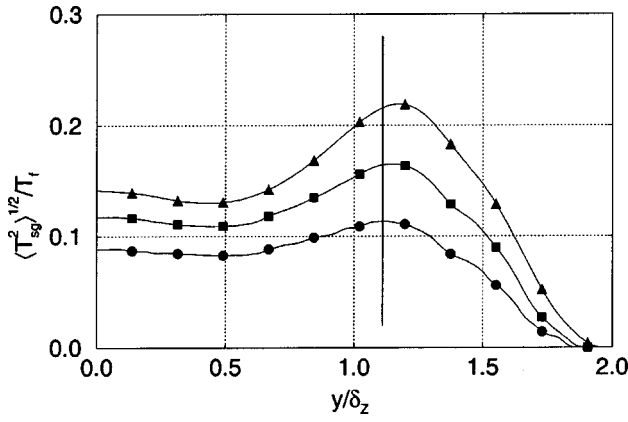
FIG. 25. Subgrid-scale temperature for Z_{st}=0.2 . Symbols denote different filter sizes \Delta_f/\Delta_g : ●, 4; ■, 8; and ▲, 16. Vertical solid line indicates position of the stoichiometric surface.
