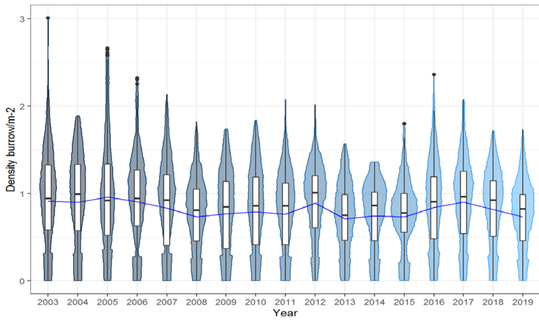
Figure 2: Times series of adjusted burrow density (Violin and box plot).
