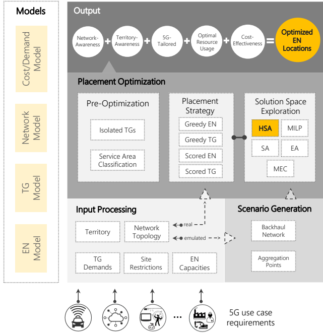
FIGURE 1: EdgeON Architecture.
