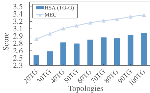
FIGURE 8: Performance results for HSA and MEC using TG-G as placement strategy.
