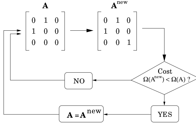
Figure 1: Basic scheme of the evolutionary algorithm used in this paper. Starting from a given signal-object matrix \mathbf{A} (here n = m = 3 ) the algorithm performs a change in a small number of bits (specifically, with probability \nu , each a_{ij} can flip). The cost function \Omega is then evaluated and the new matrix is accepted provided that a lower cost is achieved. Otherwise, we start again with the original matrix. At the beginning, \mathbf{A} is set up with a fixed density \rho of ones.
