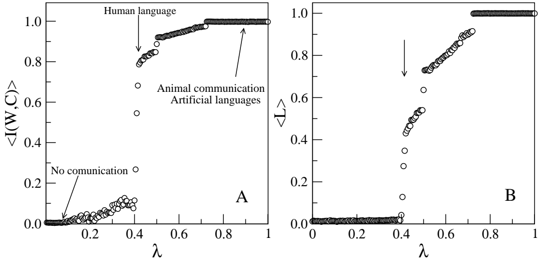
Figure 2: A. \langle I_n(\mathcal{S}, \mathcal{R}) \rangle , the average mutual information as a function of \lambda . \lambda^* = 0.41 divides \langle I_n(\mathcal{S}, \mathcal{R}) \rangle into a no communication and perfect communication phase. B. Average (effective) lexicon size, \langle L \rangle , as a function of \lambda . An abrupt change is seen for \lambda \approx 0.41 in both of them. Averages over 30 replicas, n = m = 150 , T = 2nm and \nu = 2/\binom{n}{2} .
