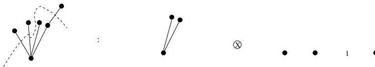
FIGURE 5. Co-product for the amputated version. The same example for the amputated version: First all tails are removed. After cutting all newly formed tails are amputated and empty trees/forests are represented by 1 = 1_K . Notice that indeed || from Figure 2 is set to 1_K as is done in the Hopf quotient.
