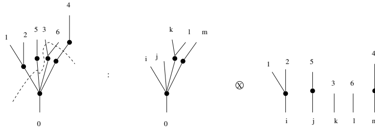
FIGURE 3. One term of the dual to \gamma as given by a cut in the labeled case. The labels i, j, k, l, m indicate the pairing of the half edges after severing the edges.
