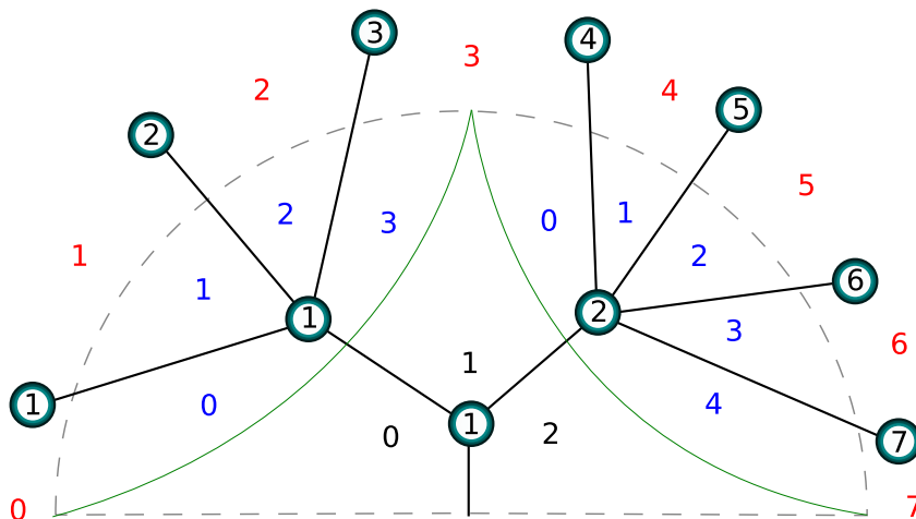
FIGURE 8. An example of a factorization \underline{7} \rightarrow \underline{2} \rightarrow \underline{1} of order preserving surjections and, reading outwards from the root to the leaves, the corresponding operad structure map \gamma_{3,4} : [2] \cup [3] \cup [4] \rightarrow [7] .
