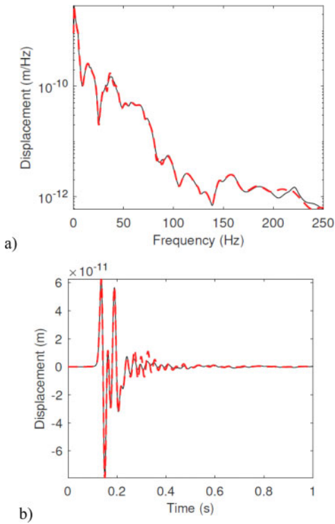
Figure 10. Vertical displacement of point P1: a) frequency domain; b) time domain. (Continuous black lines represent the results of the reference model and the dashed red lines the results of the hybrid method).
