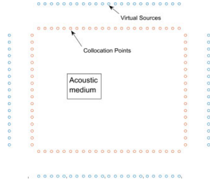
Figure 8. Collocation points and virtual sources location for the computation of re-radiated noise in the upper right enclosure of the building.
