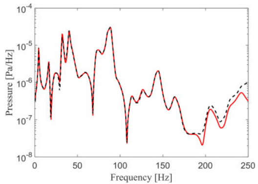
Figure 12. Frequency domain prediction of the noise pressure in center point of the upper right enclosure (Continuous red lines represent the results of the reference model and the dashed black lines the results of the hybrid method).
