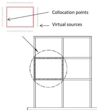
Figure 4. Schematic representation of an MFS model for the acoustic domain \Omega .
