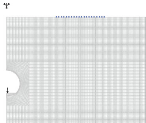
Figure 5. Tunnel-soil system 2.5D FEM-PML mesh and location of the measurement points (collocation points).
