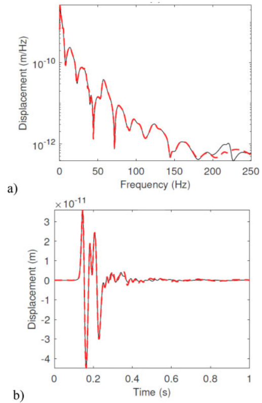
Figure 11. Vertical displacement of point P1: a) frequency domain; b) time domain. (Continuous black lines represent the results of the reference model and the dashed red lines the results of the hybrid method).
