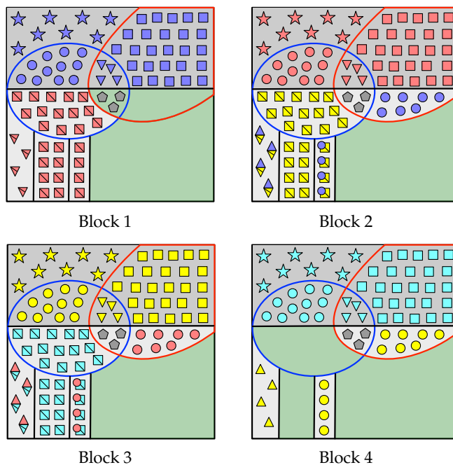
Figure 6. For Case D, graphical representation of the encoding that leads to the construction of \tilde{A}_{1:L}[\mathcal{H}_V^{(n)}] when L = 4 . Consider the Block 2: \mathcal{R}_1^{(n)} , \mathcal{R}_2^{(n)} , \mathcal{R}_{1,2}^{(n)} , \mathcal{R}'_{1,2}^{(n)} and \mathcal{R}_\Lambda^{(n)} are those areas filled with yellow squares, blue circles, blue and yellow diamonds, yellow squares overlapped by blue circles, and gray pentagons, respectively, and the set \mathcal{I}^{(n)} is the green filled area. At Block i \in [1, L] , W_i is represented by symbols of the same color (e.g., red symbols at Block 2), and \Theta_i^{(V)} , \Psi_i^{(V)} and \Gamma_i^{(V)} are represented by squares, circles, and triangles, respectively. Furthermore, \Theta_i^{(V)} and \bar{\Gamma}_i^{(V)} are denoted by squares and triangles, respectively, with a line through them. At Block i \in [2, L - 1] , \Gamma_{1,i-1}^{(V)} \oplus \bar{\Gamma}_{1,i+1}^{(V)} is represented by diamonds, and \Psi_{2,i-1}^{(V)} \oplus \Theta_{2,i+1}^{(V)} by squares overlapped by circles. At Block i \in [1, L] , S_i is stored into those entries that belong to the green area. Sequence \Lambda_1^{(V)} is denoted by gray pentagons and is repeated in all blocks. Sequences Y_{(1)}^{(V)} and Y_{(2)}^{(V)} are the entries inside the red curve at Block 1 and the blue curve at Block L , respectively.
