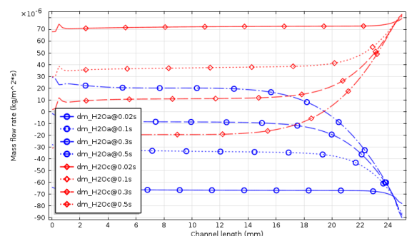
Fig. 6. Water mass flow rates across the membrane from 0 to 0.5s (0.2A/cm 2 , T FC =60°C, RH cat =65%@25°C)
