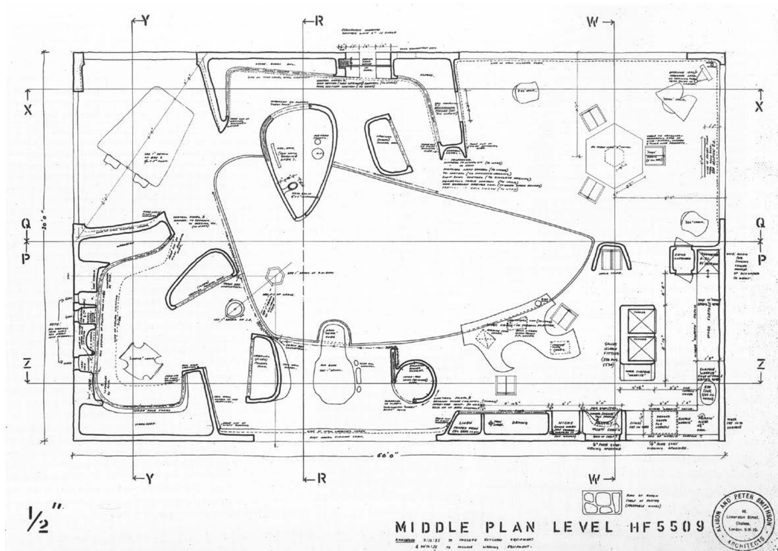
Planta de The House of the Future , Alison y Peter Smithson, 1956. Fuente: Dirk van den Heuvel y Max Risselada, Alison and Peter Smithson - from the House of the Future to a house of today , (Rptterdam: 010 Publishers, 2004), p. 82
