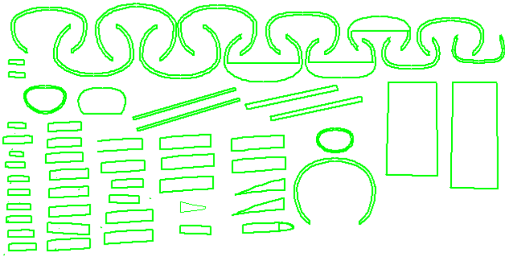
Figure 2: The DXF representing the 3mm thick plate (2)
