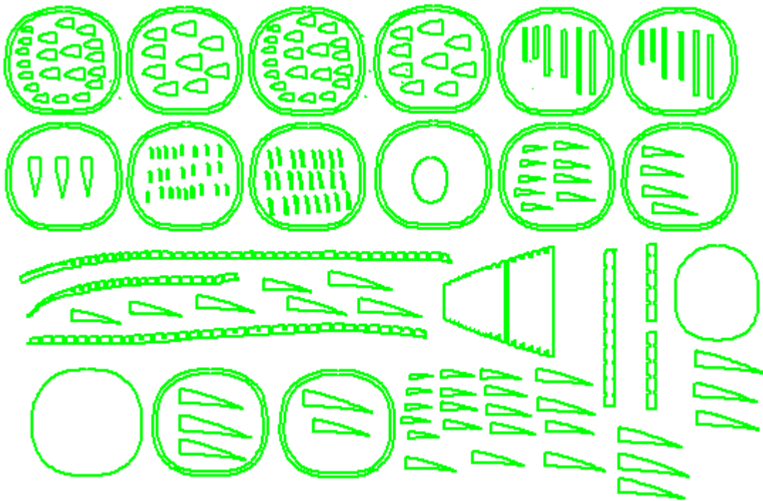
Figure 3: The DXF representing the 3mm thick plate (3)
