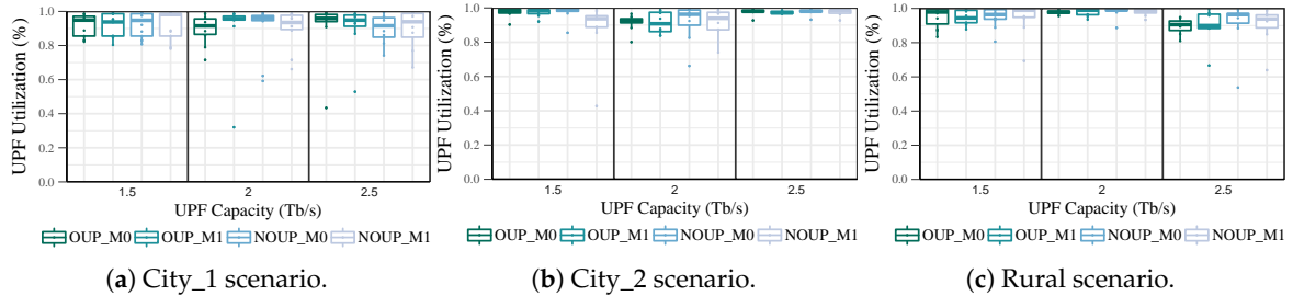
Figure 10. UPF Utilization vs. capacity for services with low requirements.
