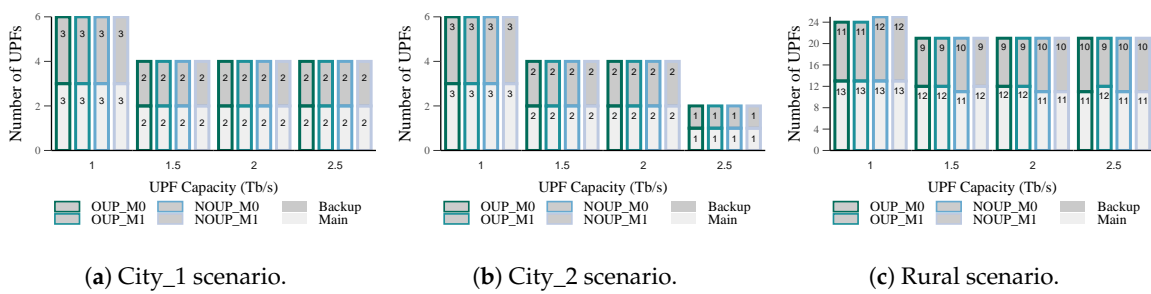
Figure 5. Number of UPFs vs. capacity for services with high requirements.
