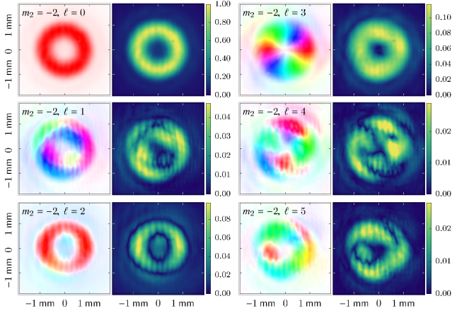
Figure S2 | Transformed experimental results. Fourier transform of the experimental results of Fig. S1, shown in both magnitude (right-hand panels) and phase (left-hand panels; \arg(\tilde{f}_\ell(x, y)) as the hue and |\tilde{f}_\ell(x, y)| as the saturation). We normalize |\tilde{f}_\ell(x, y)| to its maximum value within each plot, but we show its scale with respect to the base \ell = 0 intensity |\tilde{f}_0(x, y)| on the density-plot tick marks. Thus, the only meaningful channel \ell > 0 is \ell = 3 , with a dominant signal and a clear phase winding.
