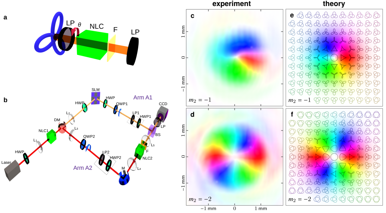
Figure 3 | Experimental configuration and results. (a) Basic scheme for nonlinear polarimetry, giving rise to (b) our experimental set-up (see the Methods section for a detailed description and definitions of the acronyms). (c,d) Experimental measurement of T_{3,3}(x, y) for m_2 = -1 and m = -2 on the 2\omega arm, taken by Fourier-transforming the CCD images as a function of the polarizer angles, shown with its amplitude |T_{3,3}(x, y)| as the saturation and the phase \arg(T_{3,3}(x, y)) , directly linked to the trefoil orientation angle, as the hue. (e,f) Theoretical prediction for the field tensor moment T_{3,3}(x, y) of a gaussian and a Laguerre-Gauss beam with m_2 = -1 and m = -2 , showing a clear match to the corresponding measurements, overlaid with the Lissajous figures of the polarization at different points around the beam. At the center of the beam the Lissajous figure is a circle, and it shifts to a triangle and then a trefoil as the probe point gets further from the axis – but the orientation of the deformation away from circularity depends on the direction of departure from the axis.
