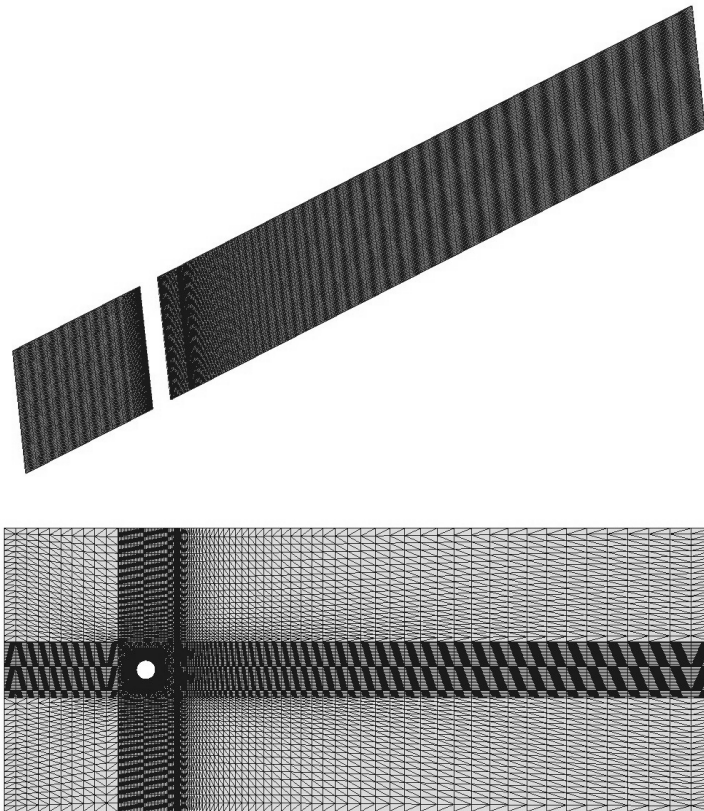
Figure 12. Flow past a cylinder. Details of the mesh used for the computations
