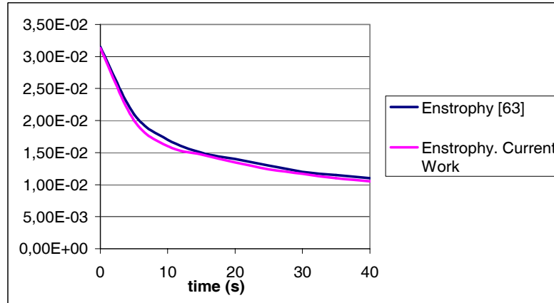
Figure 10. Enstrophy evolution with time
