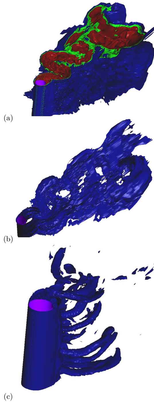
Figure 14. Vorticity vector modulus \omega isosurfaces. (a) \omega = 0.1, 0.2, 0.3 ; (b) \omega = 0.2 ; (c) \omega = 2
