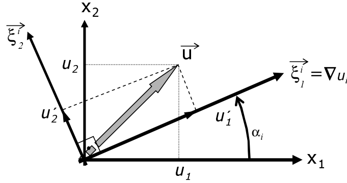
Figure 6. Definition of the principal curvature direction \bar{\xi}_1^i along the gradient of u_i
