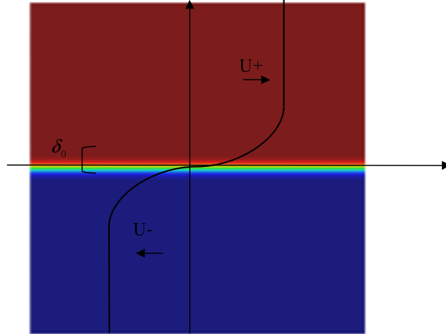
Figure 8. Initial configuration for the 2D mixing layer problem
