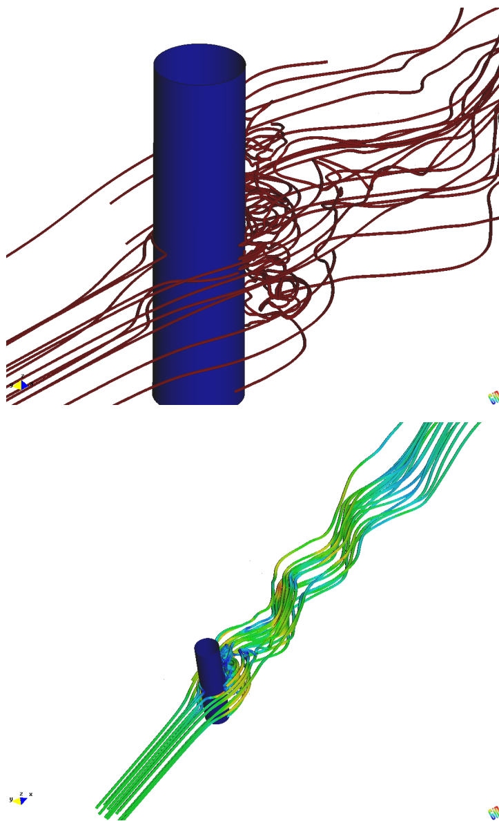
Figure 15. Streamlines at time t = 50
