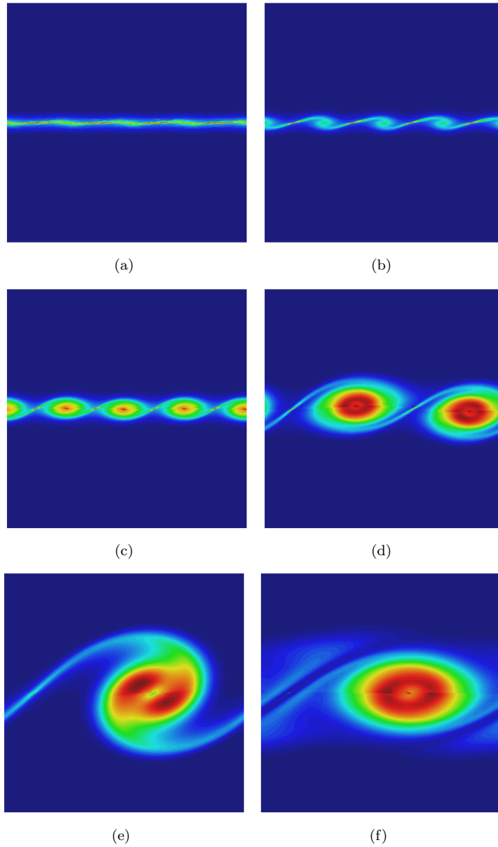
Figure 9. Vorticity modulus contours at times 0.5 (a), 0.75 (b), 1 (c), 2 (d), 3 (e) and 4s (f)
