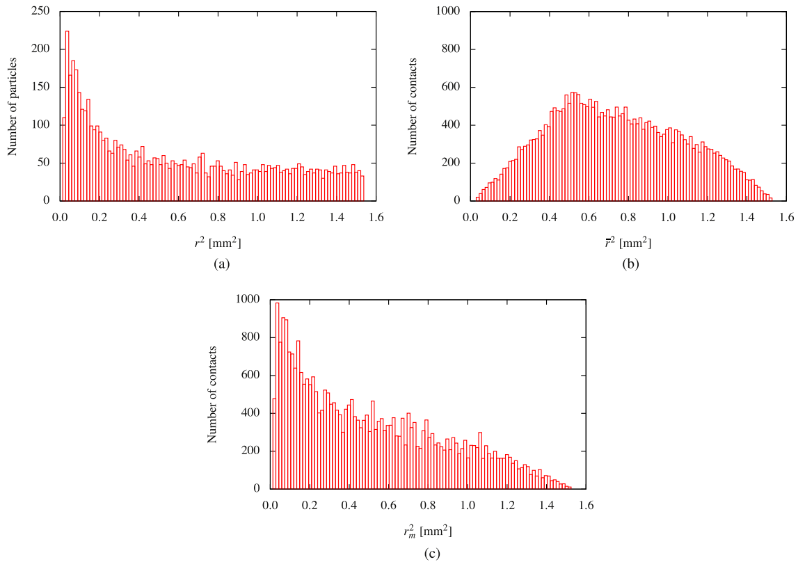
Fig. 9. Distribution of the squares of the characteristic geometric parameters for the specimen 2: (a) distribution of the particle radius squares r^2 , (b) distribution of the squares of the arithmetic means of the contacting particle radii \bar{r}^2 , (c) distribution of the squares of the minimum radii of the contacting particles r_m^2 .
