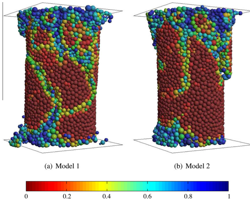
Fig. 11. Damage in the models with local evaluation of the parameters – simulation results for the specimen 1.
