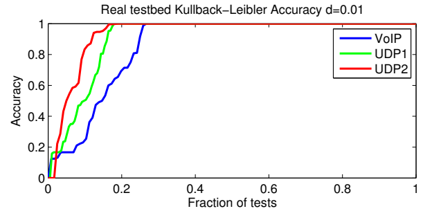
(a) Kullback-Leibler Divergence Accuracy
