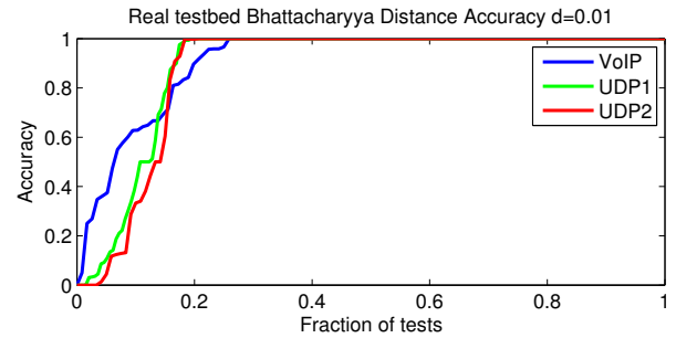
(b) Bhattacharyya Distance Accuracy
