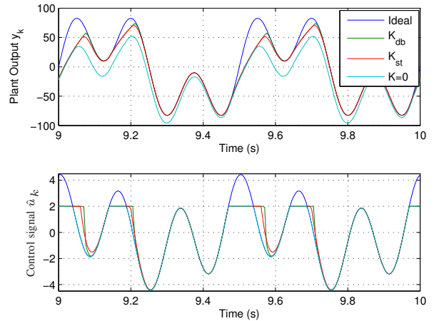
Fig. 6. Steady state saturation behaviour.
