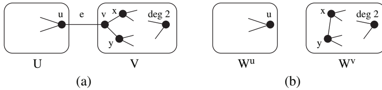
FIG. 2. (a) A bridge e = \{u, v\} in an almost 3-regular graph G with components U and V of G - \{e\} . (b) Graphs smaller than G from which we obtain a partition into trails W^u and W^v .
