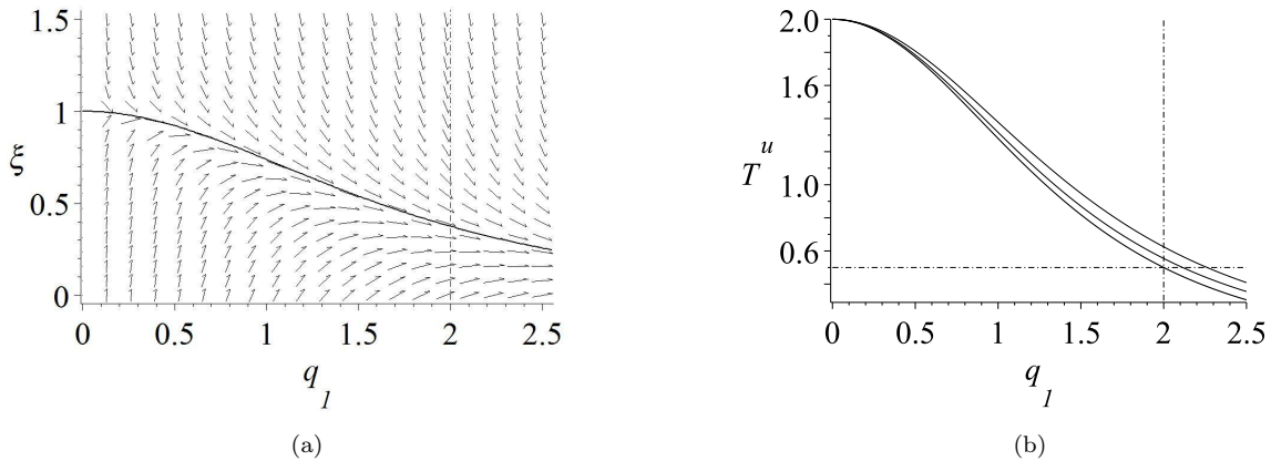
Figure 1: (a) Direction field corresponding to the Riccati equation (53), where the solution with \xi(0) = \mu := \lambda_2 - \lambda_1 , for \lambda_2 = 2 , \lambda_1 = 1 , is also plotted. (b) Three solutions of the Riccati equation (53) for \lambda_2 = 2 : the lowermost one corresponds to \lambda_1 = 2 and the other two, in ascending order, to \lambda_1 = 1.75 and \lambda_1 = 1 , respectively. Note that the corresponding to \lambda_1 = \lambda_2 = 2 , holds the point (2, \lambda_1/4) = (2, 1/2) .
