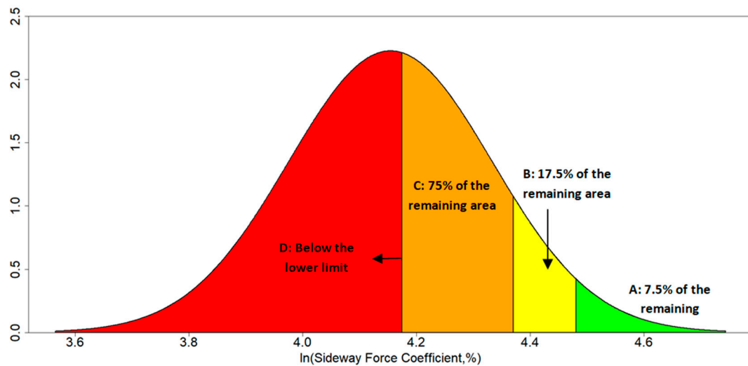
Figure 6. Probability density function of skid resistance.
