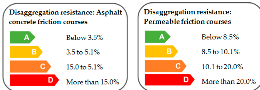
Figure 14. Disaggregation resistance labels based on the type of mixture.
