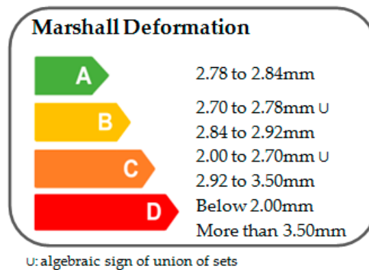
Figure 13. Marshall deformation global label.
