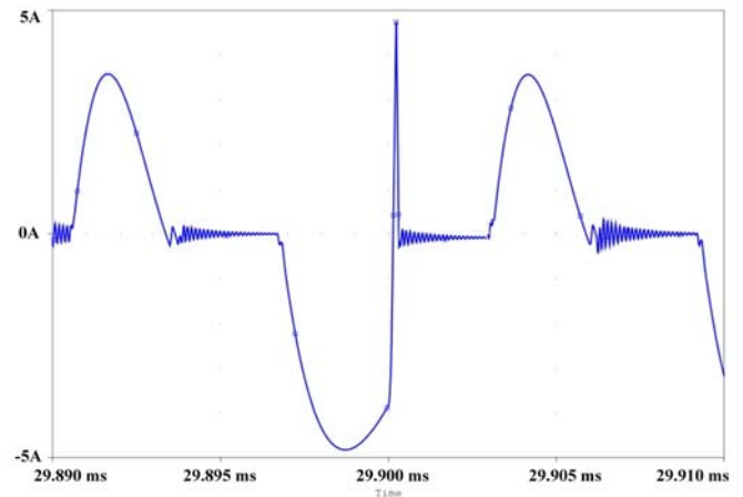
(d): Current waveform of L_1
