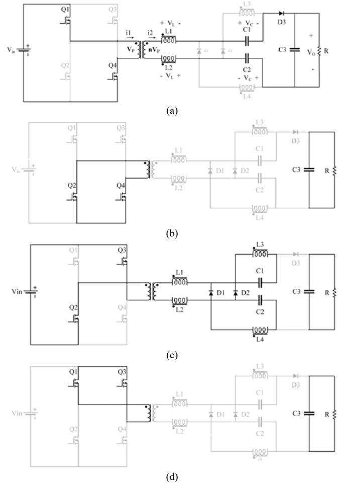
Fig. 2. Equivalent circuits of the proposed converter
