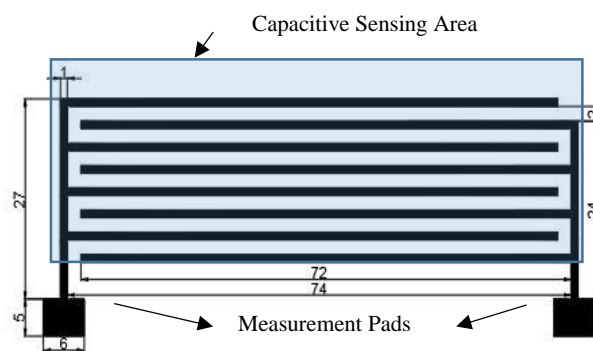
Figure 1. Layout and dimension detail of the proposed moisture sensor (in mm). The bottom squares correspond to the characterization pads, and the capacitive sensing area corresponds to the interdigitated area.
