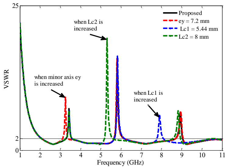
Figure 10. Parametric study of the resonator.
