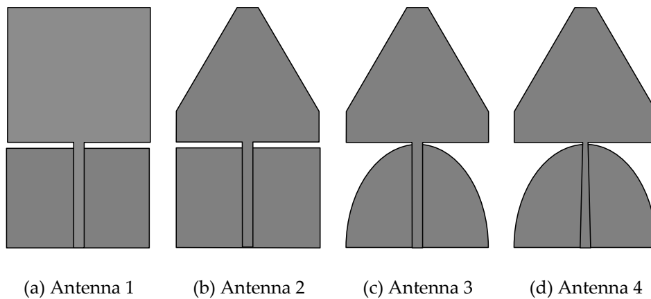
Figure 1. The geometry of a super-wideband (SWB) antenna with: (a) Rectangular ground and radiator; (b) rectangular ground and trapezoid radiator; (c) trapezoid radiator and semicircular ground; (d) semicircular ground, trapezoid radiator, and rectangular tapered feed.
