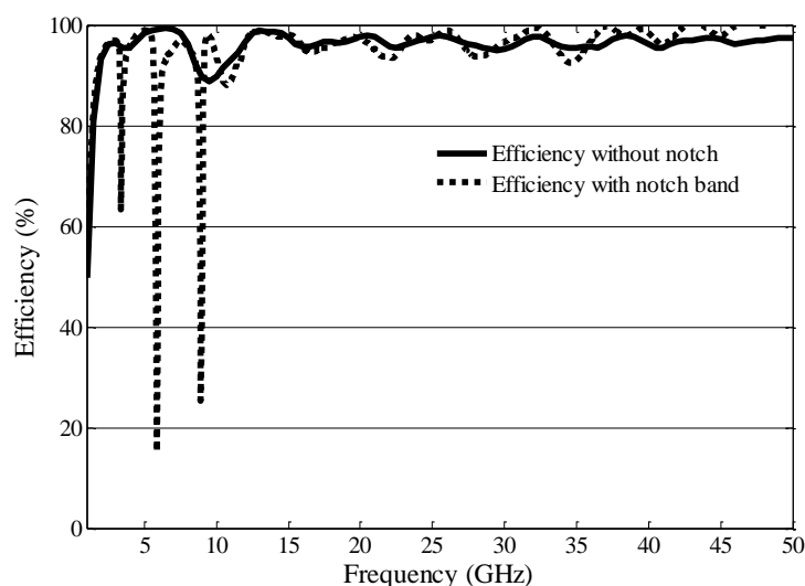
Figure 14. The plot of efficiency plot without and with notch bands.
