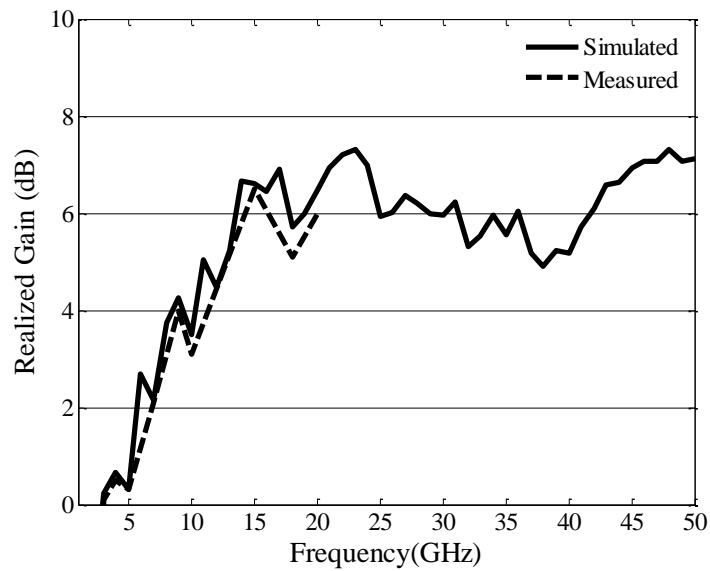
Figure 6. The simulated and measured peak gain.
