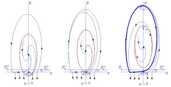
Figure 3: Periodic orbit of the regularized family Z_{\mu,\epsilon} when X_\mu^+ has a repelling periodic orbit \Gamma_\mu (the red dotted orbit). For \mu < 0 and \mu = 0 the regularized system has no periodic orbits. For \mu > 0 the regularized system has a periodic orbit \Gamma_{\mu,\epsilon} which coexists with \Gamma_\mu . A bifurcation of periodic orbits in the regularized system corresponding with the grazing-sliding bifurcation in the Filippov system can occur.
