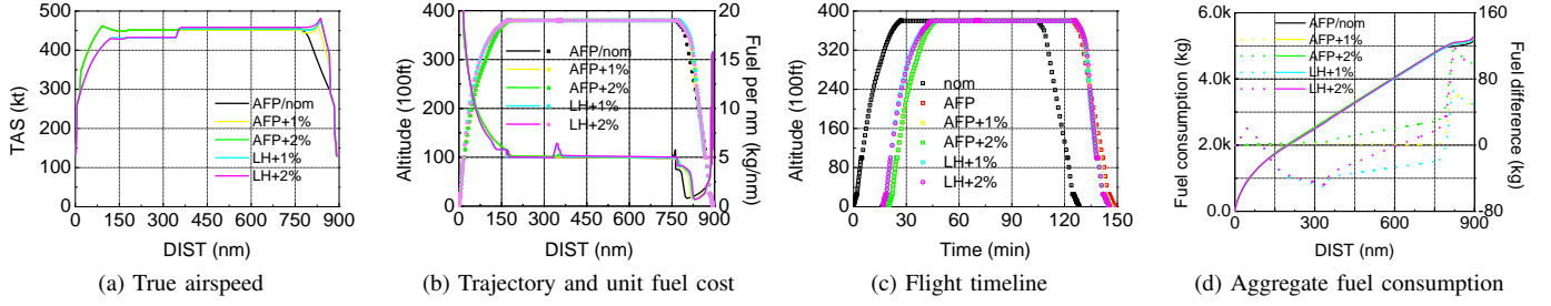
Fig. 6: Comparison between the AFP and LH trajectories (with 1% and 2% of extra fuel allowances)
