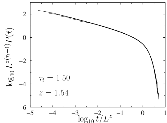
Fig. 3. Data collapse analysis of the integrated avalanche time distribution for the conserved RD model in d = 2 . System sizes L = 64, 128, 256, 512 , and 1024 .
