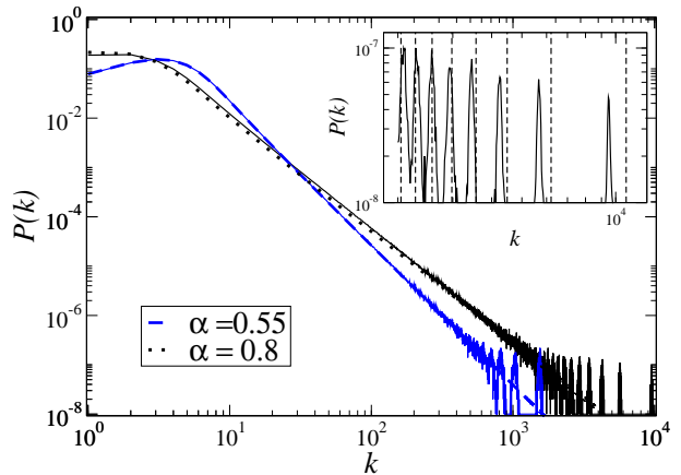
Fig. 2. Degree distribution in the SM for two different values of \alpha . The dotted and dashed lines represent the theoretical value given by Eq. (35). In the inset: enlargement of the tail of the distribution. Peaks due to the discretization of the degree are visible. Dashed vertical lines represent the theoretical values of the centers of such peaks.
