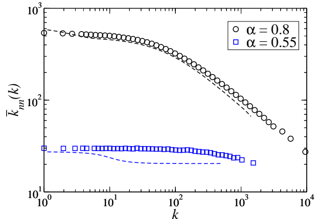
Fig. 4. Average nearest neighbor degree of the vertices with degree k , in the SM for two different values of \alpha . The dashed lines correspond to the numerical summation of Eq. (39).
