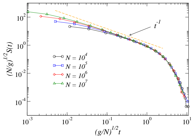
FIG. 6: Scaling of the survival probability S(t) for \gamma = 2.5 and \omega = \gamma - 1 in a single instance network.
