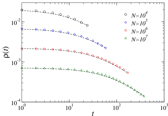
FIG. 5: Evolution of the concentration \rho(t) in region II for different network sizes, \gamma = 2.5 , and \omega = 2 . The initial concentration is \rho_0 = \langle k \rangle / 2k_c and results are averaged over 500 realizations. Dashed lines correspond to the theoretical prediction Eq. (41).
