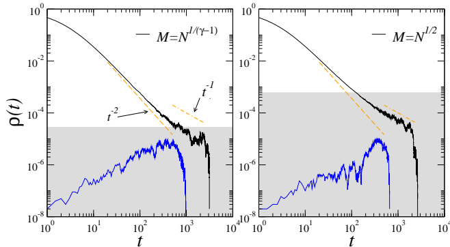
FIG. 2: Example of two different types of experiment to study the CP dynamics at criticality performed in an annealed network of size N = 10^8 , \gamma = 2.5 , and m = 2 . The top (black) curve is the density decay starting from a fully active network. The bottom (blue) curve corresponds to a spreading experiment starting from a single active vertex. The left plot corresponds to the hard cutoff M = N^{1/(\gamma-1)} and the right plot to M = N^{1/2} . Grey areas depict the values of \rho in the domain \rho \in [N^{-1}, \langle k \rangle k_c^{-1}] . In all cases trajectories are for a single run in an instance network.
