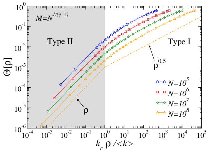
FIG. 1: Numerical evaluation of the function \Theta[\rho] as a function of k_c \rho / \langle k \rangle for different network sizes. The degree exponent is \gamma = 2.5 and we use \omega = \gamma - 1 . In the type II region, it is clearly visible a linear behavior, in agreement with Eq. (34). In the type I region, convergence towards the theoretical expression given by Eq. (34) is much slower.
