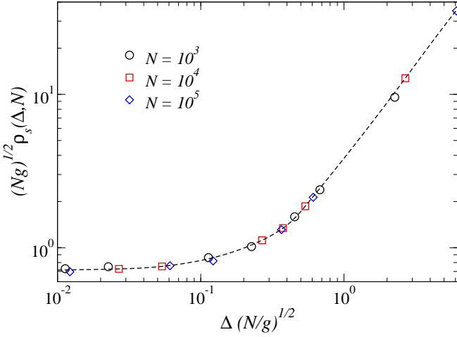
FIG. 7: Scaling of the density for surviving runs for \gamma = 2.2 and \omega = 2 . Each point is the result 10^2 realizations of the stochastic process on each of the 10^2 network realizations. The dashed line is an interpolation of the data as a guide to the eye.
