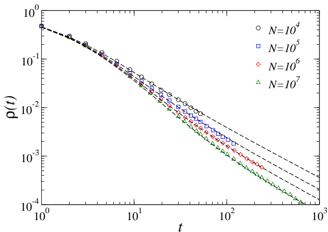
FIG. 3: Evolution of the concentration \rho(t) starting from a fully infected network for different network sizes, \gamma = 2.5 , and \omega = 2 . Results are averaged over 100 realizations in a single instance network. Long dashed lines correspond to the numerical solution of the set of Eqs. (12), using as input the empirical degree sequence used in the simulations. The very nice agreement between both sets of curves justifies our approximation.
