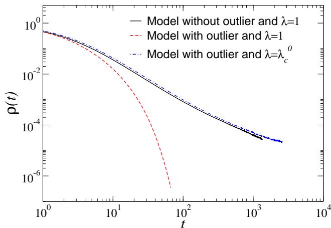
FIG. 8: Density decay starting from a fully active network for the model with and without outlier. Network size is N = 10^8 , \gamma = 2.5 , and M = N^{1/2} . Results are averaged over 100 realizations in a single instance network.
