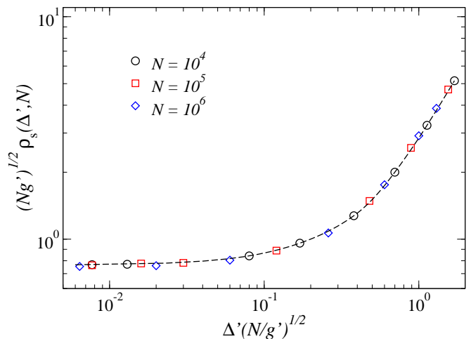
FIG. 9: Scaling of the density for surviving runs for \gamma = 2.5 and \omega = 2 , with an outlier of degree k_{out} = N . Each point is the result of 10^4 realizations of the stochastic process on a single network realization. The dashed line is an interpolation of the data as a guide to the eye.
