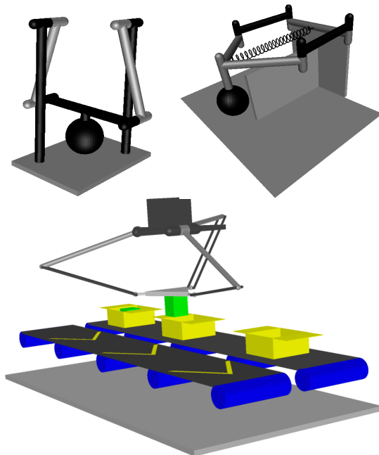
Fig. 4. Test cases used to validate the planner: a four-bar pendulum (top, left), a five-bar robot (top, right), and a Delta robot (bottom).
