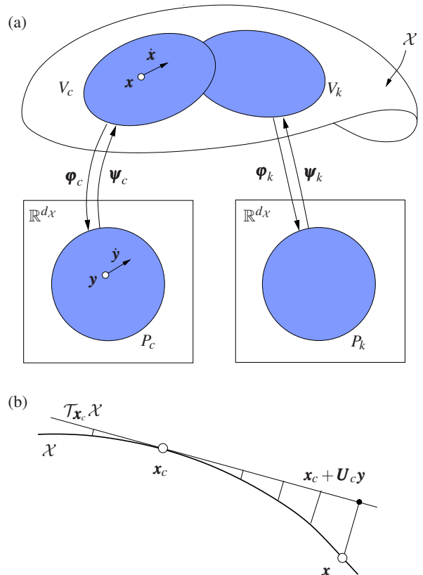
Fig. 2. (a) An atlas is a collection of maps \boldsymbol{\varphi} providing local coordinates to all points of \mathcal{X} . (b) The projection of the points \mathbf{x} \in \mathcal{X} to \mathcal{T}_{\mathbf{x}_c} \mathcal{X} leads to specific instances of \boldsymbol{\varphi}_c and \boldsymbol{\psi}_c .
