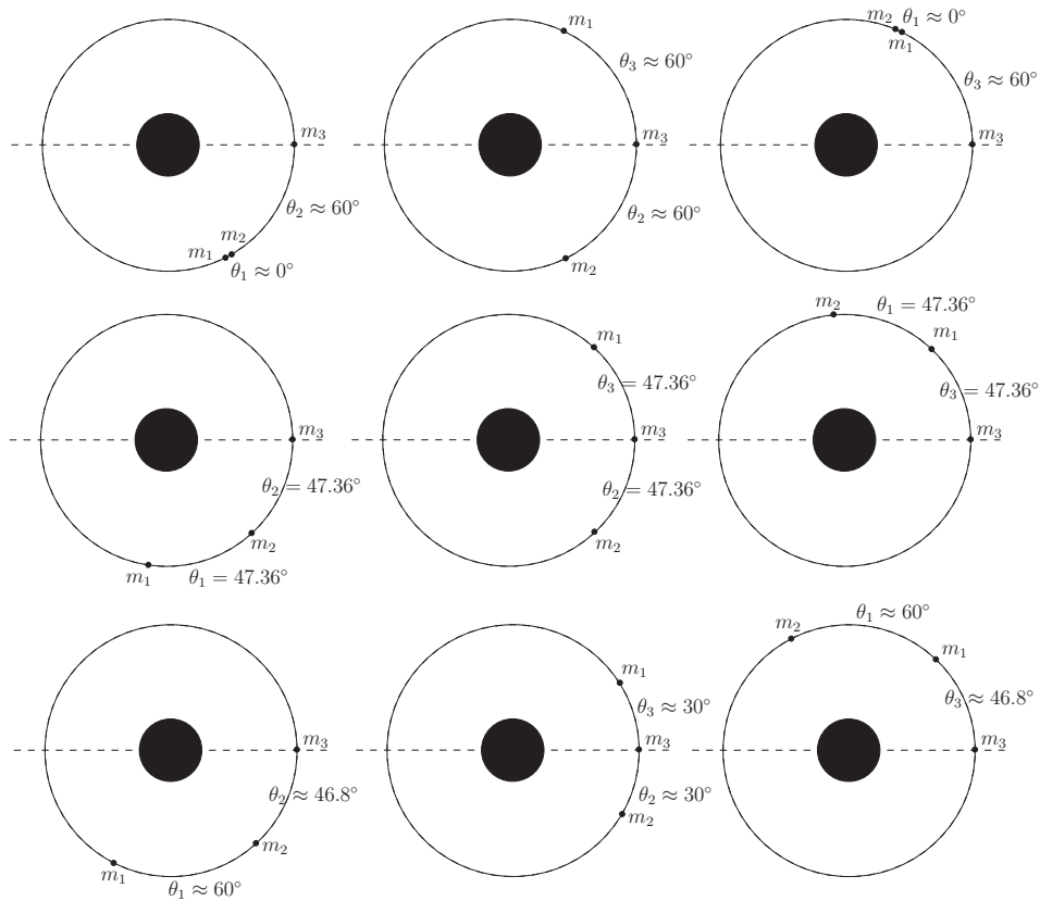
Figure 3. Coorbital central configurations of class A for different values of \mu . Top \mu \approx 0 , middle \mu = 1 and bottom \mu \gg 1 . Left A_1 , center A^s and right A_2 .
