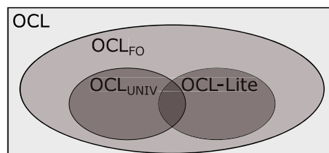
Fig. 8 Relation of different OCL fragments
