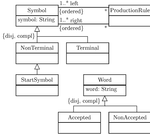
Fig. 3 UML class diagram for a 0 type grammar
