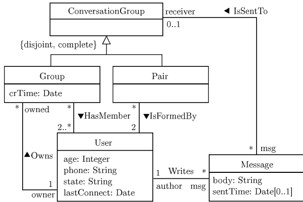
Fig. 1 UML class diagram
