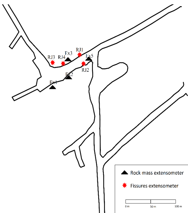
Figure 4. Scheme of the Minilla mine with the extensometers location. Source: Authors.
