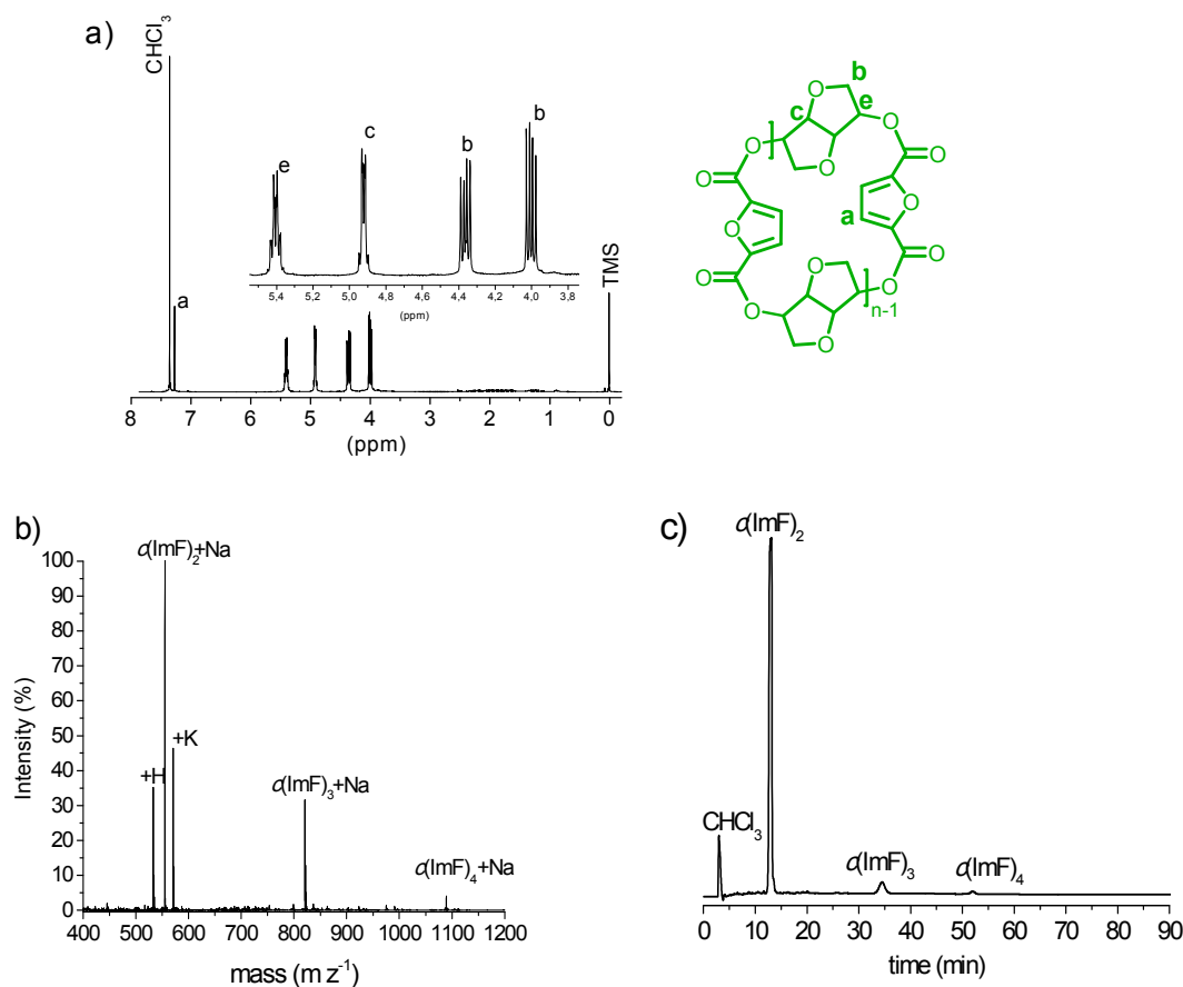
Figure 1. a) 1 H NMR, b) MALDI-ToF, and c) HPLC of c(ImF) n after purification.
