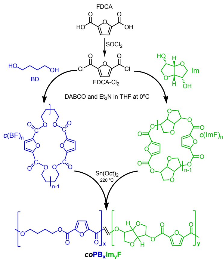
34 Scheme 1. Synthetic route to poly(butylene- co -isomannide 2,5 furandicarboxylate) 35 copolyesters.
