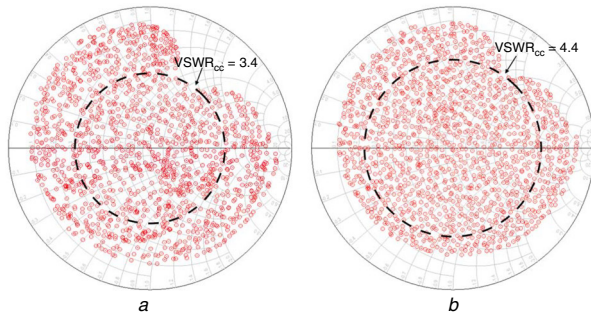
Fig. 6 Simulated and measured tuner coverage ( S_{11} ) at 1.4 GHz a Measured tuner states b Simulated tuner states
