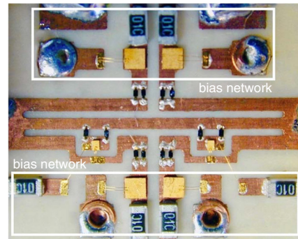
Fig. 3 Picture of fabricated TLM tuner
