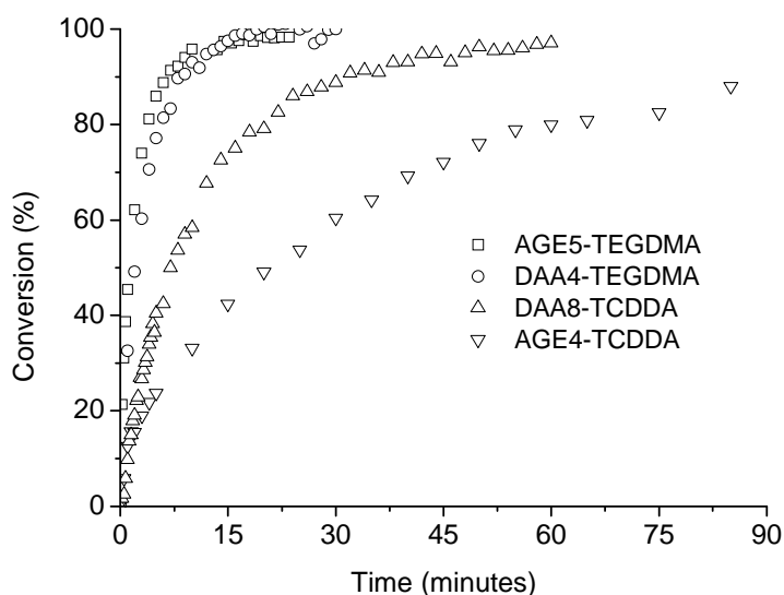
Fig 2. Stage 1 (thiol-Michael) acrylate/methacrylate FTIR conversions of all four comonomer - Michael acceptor pairs. Michael donor is pentaerythritol tetrakis(3-mercaptopropionate) (S4). Reaction is carried out at 40°C.
