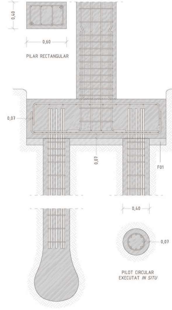
PILOT CIRCULAR EXECUTAT IN SITU
