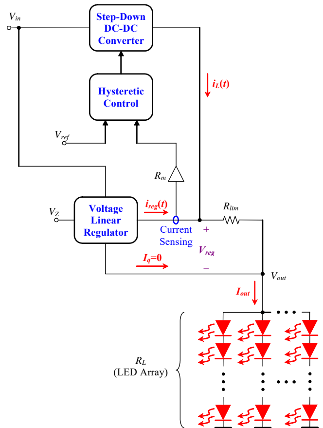
Fig. 4. Block diagram of the proposal of the linear-assisted DC/DC regulator-based current source that supplies a LED array.
