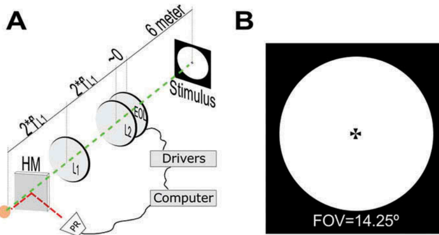
Figure 1. A: schematic view of the setup. B: accommodative stimulus used in the experiment. HM: Hot mirror. EOL: Electro-optical lens. PR: PowerRef II. f : focal length.
