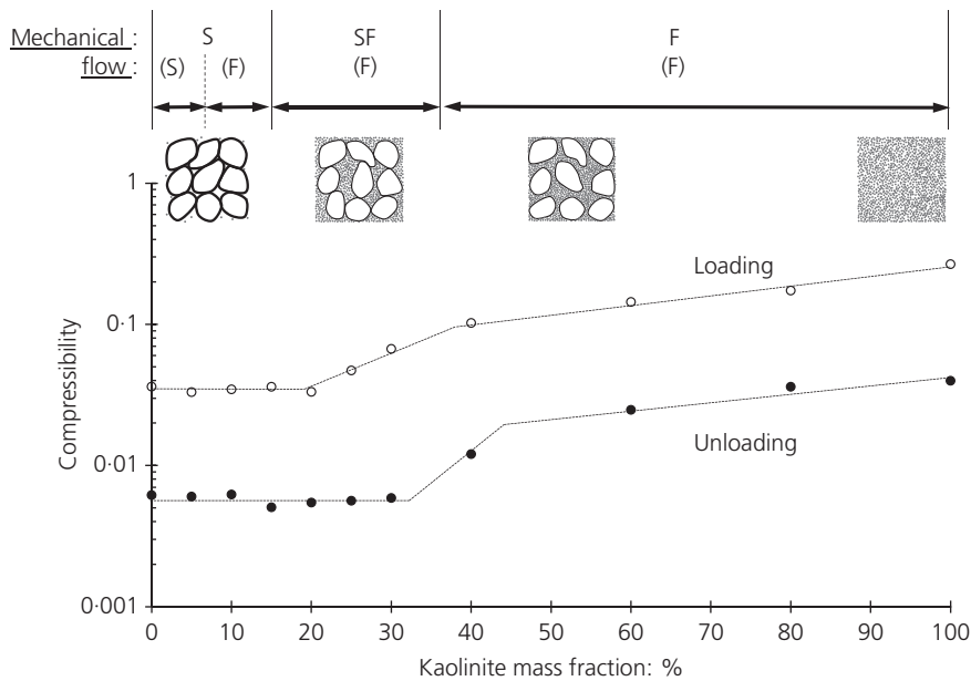
Fig. 2. Compressibility during loading and unloading against kaolinite mass fraction. Compressibility computed as C = \Delta e / \log[(\sigma'_0 + \Delta\sigma')/\sigma'_0] . The RSCS shown at the top of the figure recognises the fraction that controls the mechanical behaviour and the fraction that controls fluid flow (respectively, the first and second letter in parenthesis), refer to Park & Santamarina (2017)
