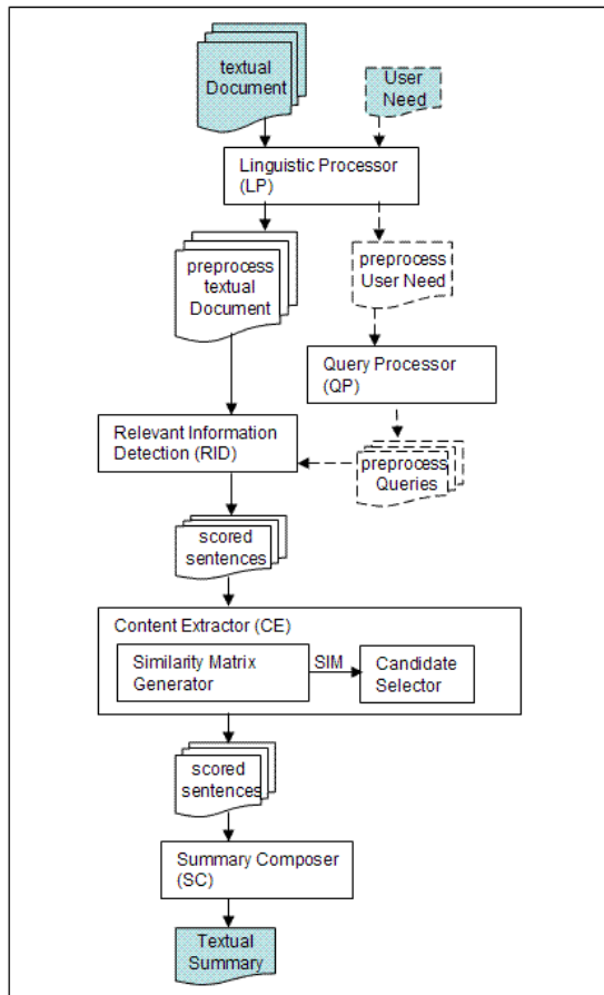
Figure 1: FEMsum data flow
