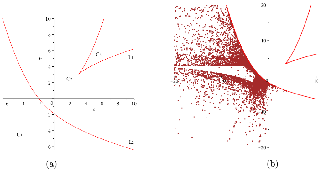
Figure 1. (a) Connected components L_1 and L_2 of the curve R(a, b) = 0 , and regions C_1 , C_2 and C_3 of the plane. (b) 10000 iterates of an orbit with initial condition in C_3 .
