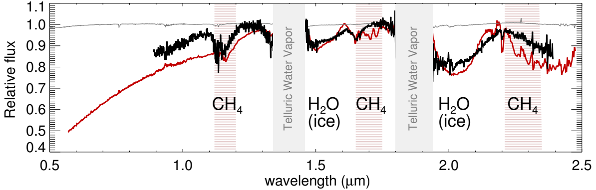
Fig. 5.— The transmission spectrum of Jupiter as measured with the WHT telescope (black line) during the umbral phase. Gray shaded regions mark the deeply absorbed telluric bands of \text{H}_2\text{O} , which cannot be observed from the ground. As in Figure 2, the thin gray line is the brightness ratio of the light reflected off Ganymede when fully illuminated by the Sun at two different airmass. Overplotted (red line) is one of Jupiter’s umbral spectra taken with the VLT. Note how both WHT and VLT spectra shown the fingerprints of gaseous \text{CH}_4 and \text{H}_2\text{O} ices.
