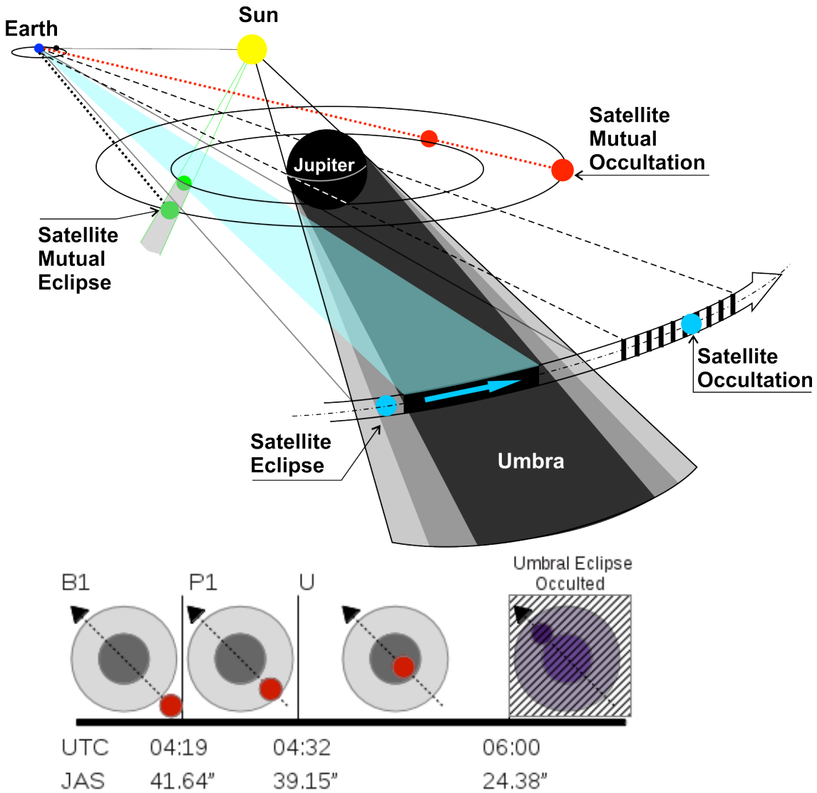
Fig. 1.— Top: A not-to-scale diagram showing the orbital geometry of the Jovian System during the observations. These events are observable from the ground when the Earth is near quadrature. The ratio spectra of Ganymede when in the umbra (or penumbra) and when fully sunlit, results in the determination of the transmission spectrum of Jupiter. Bottom: Universal time (UTC) and Angular Separation from Ganymede center to Jupiter center (JAS) for the eclipse of the satellite on 18/11/2012, as seen from Paranal, Chile.
