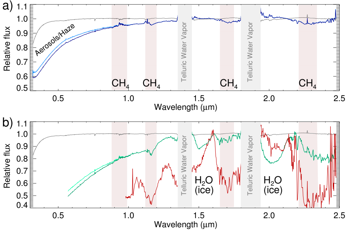
Fig. 2.— The transmission spectrum of Jupiter during the penumbra (panel a) and the umbra (panel b) phases. Gray shaded regions mark the deeply absorbed telluric bands of H_2O , which cannot be observed from the ground. The locations of the major CH_4 absorption bands are marked with a brown background shadow. On both panels, the thin gray line is the brightness ratio of the light reflected off Ganymede when fully illuminated by the Sun at two different airmass (equivalent to the airmass difference for the two spectra used to extract the transmission spectrum). It serves to illustrate the contamination from telluric lines to be expected during our measurements. All spectra have been binned to a lower resolution for display purposes. Panel a): Two of our penumbra spectra, taken at different airmass, which are almost identical except for the stronger effect of Jupiter’s haze absorption as the eclipse progresses. Panel b): Three measured umbra spectra, normalized to have unity flux at 1.6 \mu m . The different relative depth of the bands is due to different timing within the eclipse umbra, which allows probing different altitudes in Jupiter’s upper atmosphere. The first two spectra (green) show features of gaseous CH_4 and H_2O ices, while in the third spectrum (red), the H_2O ice features diminish indicating that we are probing below the H_2O ice cloud layer. In the third, deep umbra spectra the spectrum is dominated by the CH_4 absorption and by the haze.
