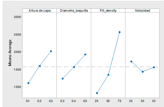
Fig. 4. Main effects plot for means of number of cycles until failure.
