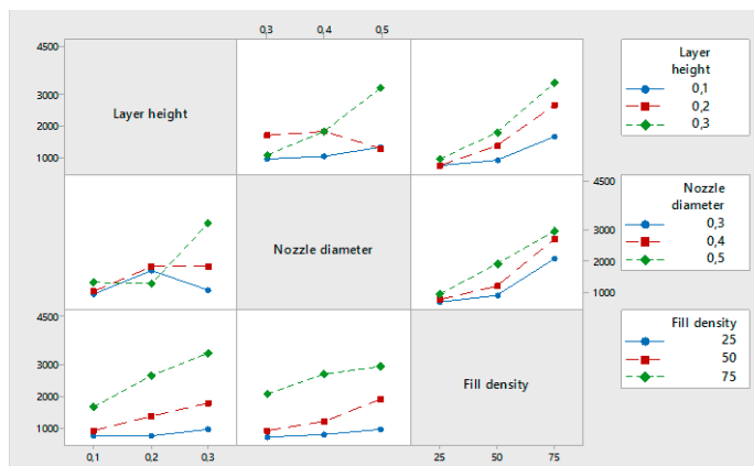
Fig. 5. Interaction plot for means of number of cycles until failure.
