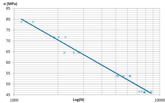
Fig. 9. S-N or Wöhler curve associated to the optimal configuration of manufacturing parameters.
