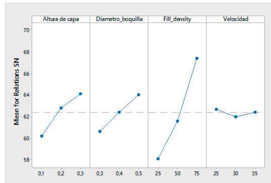
Fig. 6. Signal-to-noise ratios of each factor.
