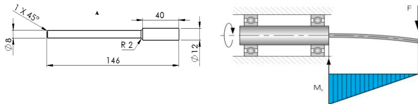
Fig. 1. (a) Dimensions of fatigue specimens ; (b) Fatigue test diagram, and maximum bending moment at the fixed section of the workpiece.
