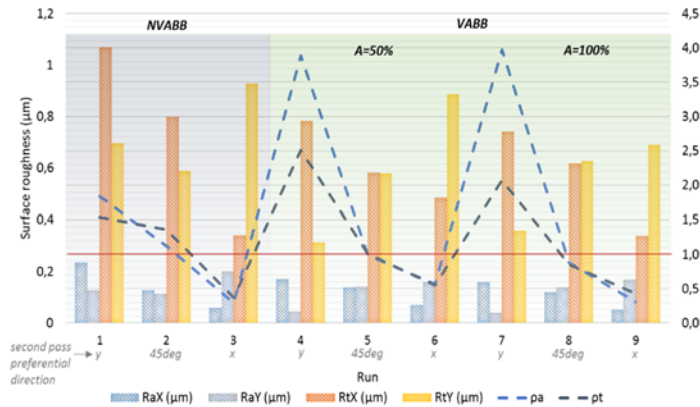
Fig. 3. Surface roughness results for all tested conditions. Blue tones show the average roughness results. Orange tones show total roughness. Red line represents \rho = 1 .
