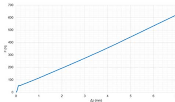
Fig. 2. Calibration curve of the burnishing tool. It fits to a linear equation according to Hooke's Law.
