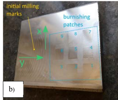
Fig. 1. (a) Initial roughness measured at the workpiece surface; (b) Burnished workpiece and reference directions referred to in this article.
