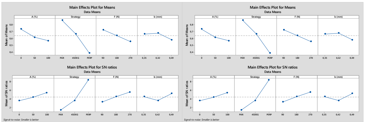
Fig. 5. Effect plots for means and S/N ratios. (a) Response variable: R_{t,x} ; (b) Response variable: R_{t,y} .
