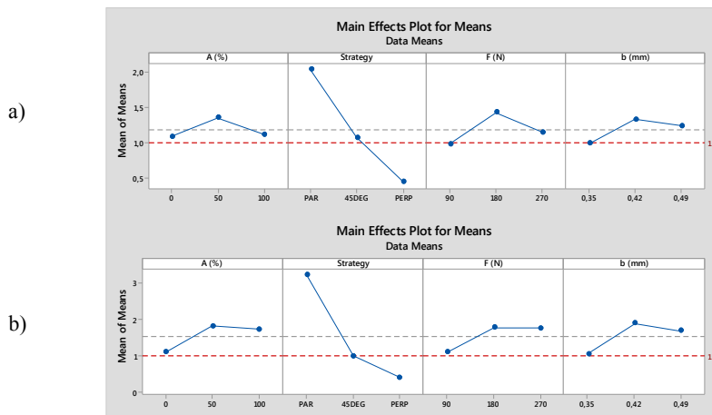
Fig. 6. Effect plots for means and S/N ratios. Response variable: (A) \rho_a , (B) \rho_t .
