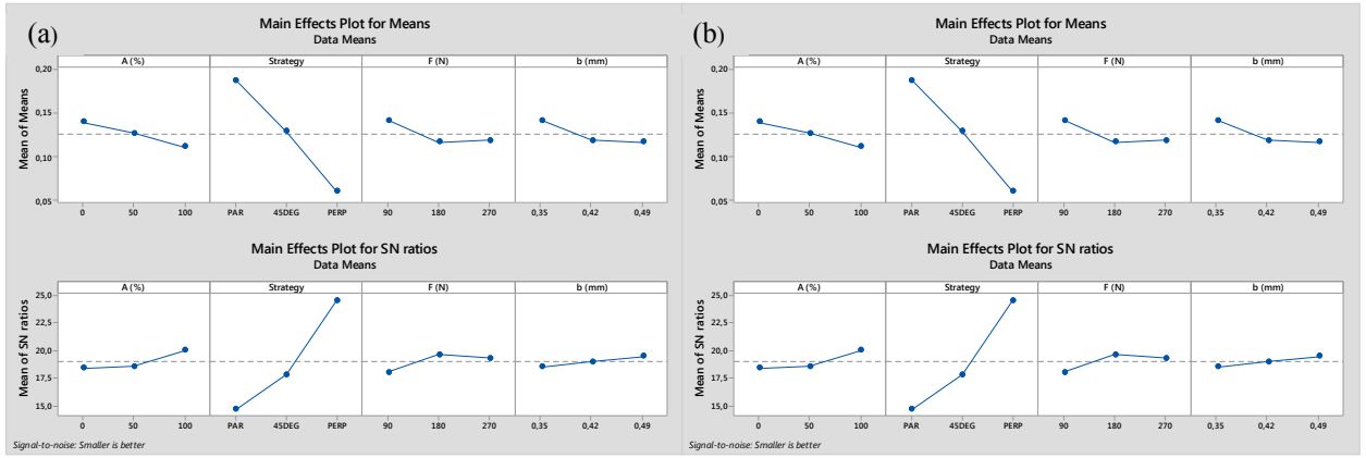
Fig. 4. Effect plots for means and S/N ratios. (a) Response variable: R_{a,x} ; (b) Response variable: R_{a,y} .
