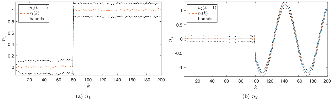
Fig. 1. Actuator-fault estimation results
